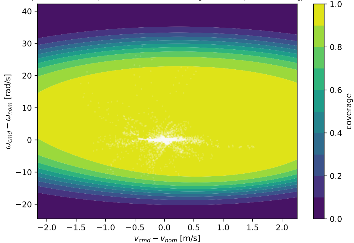
Residual coverage vs command offset (0 = off / OOD; state fixed at mean [0.38 m/s, 0.04 rad/s])
